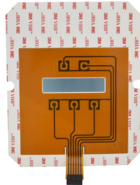
FPC Circuit Membrane Keypad
